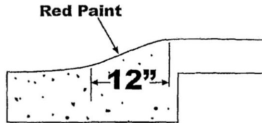
Rolled Curb
